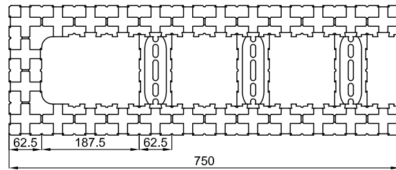
25er-Endelement (75 + 50 cm)
