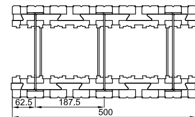
25er-Schalldämmelement
